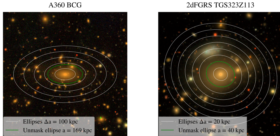
FIGURE 1: Lupton color image of the BCG of A360 and 2dFGRS TGS323Z113 in g, r, i bands from LSSTComCam data. We overlay ellipses with appropriate spacing for visual aid and show the unmask ellipse in green.
