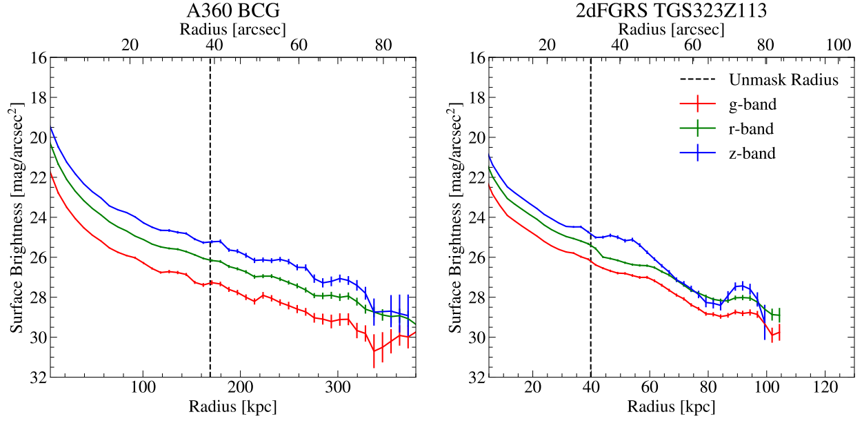
FIGURE 2: The surface brightness profile in g , r , z bands for the BCG of Abell 360 and 2dFGRS TGS323Z113. For the BCG of Abell 360 (2dFGRS TGS323Z113), the Rubin LSSTComCam data can go as deep as 30 \text{ mag/arcsec}^2 ( 28 \text{ mag/arcsec}^2 ) in the r -band.
