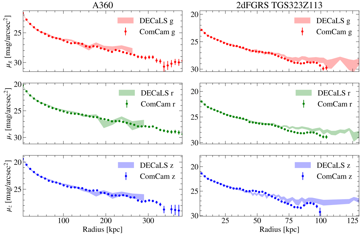
FIGURE 3: The comparison of surface rightness profiles from LSSTComCam and DECaLS. The surface brightness profiles agree well in the center, while the LSSTComCam data can go deeper in the outskirts.
